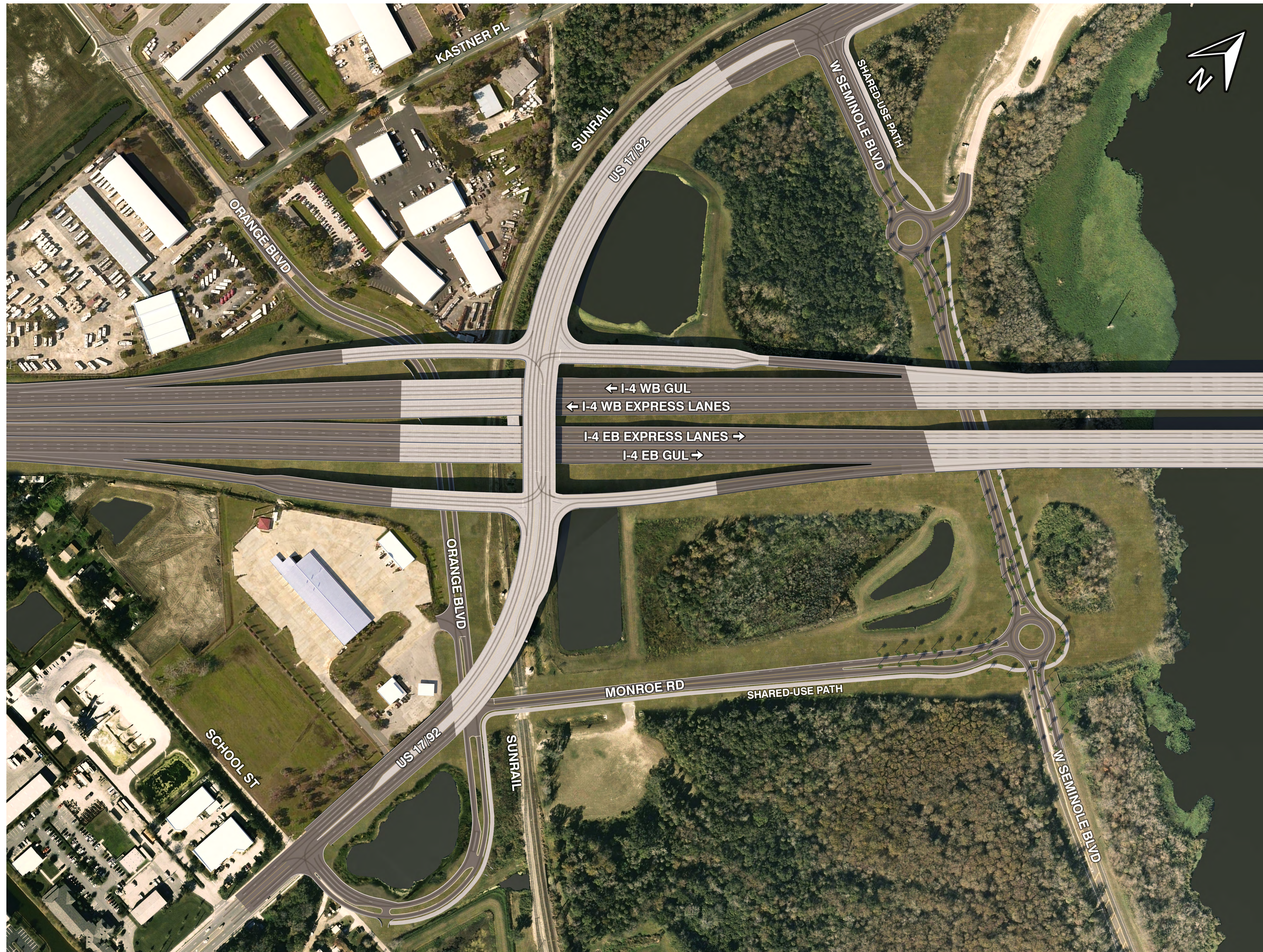
Top View
