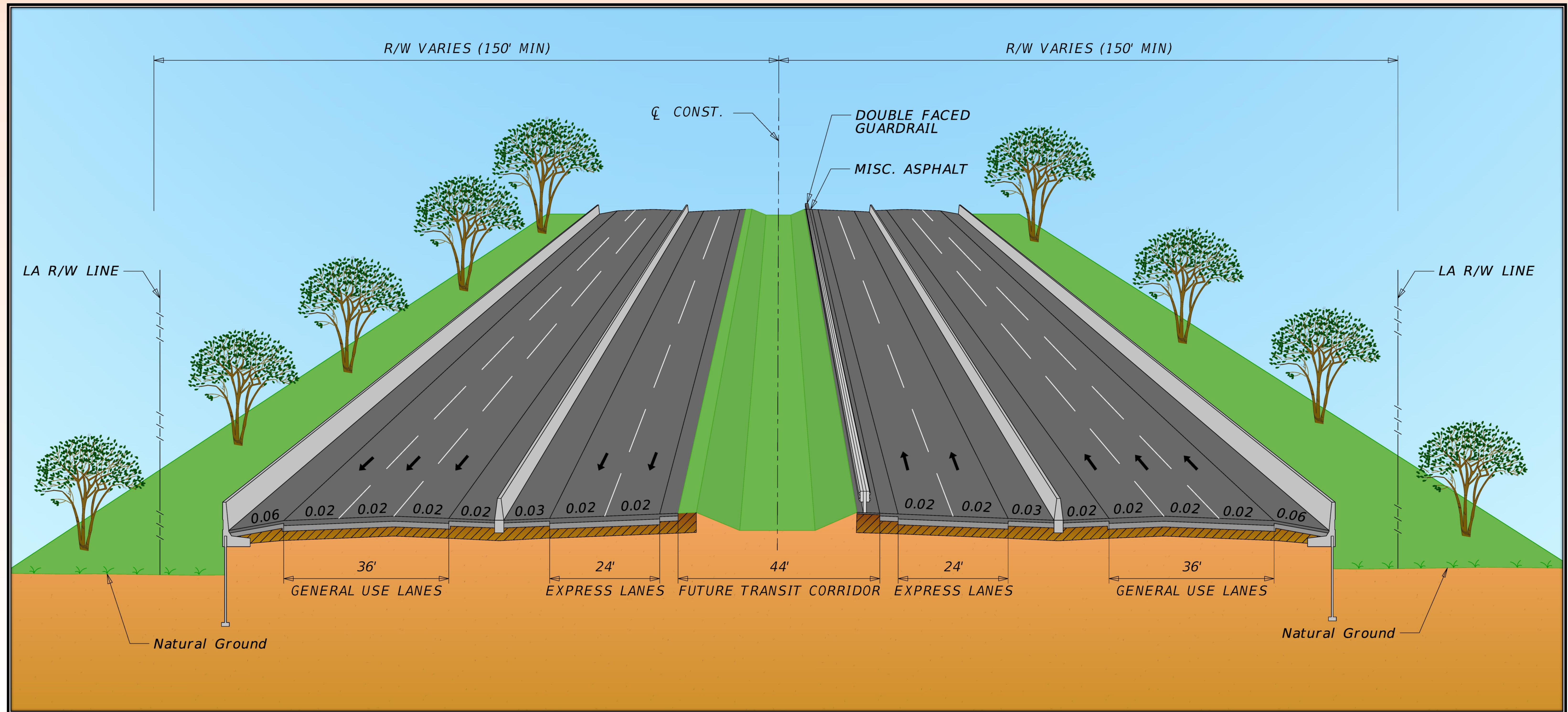
From East of US 17/92 to East of SR 472 (Design Speed = 70 MPH) 6 General Use Lanes + 4 Express Lanes (with Transit Corridor)
