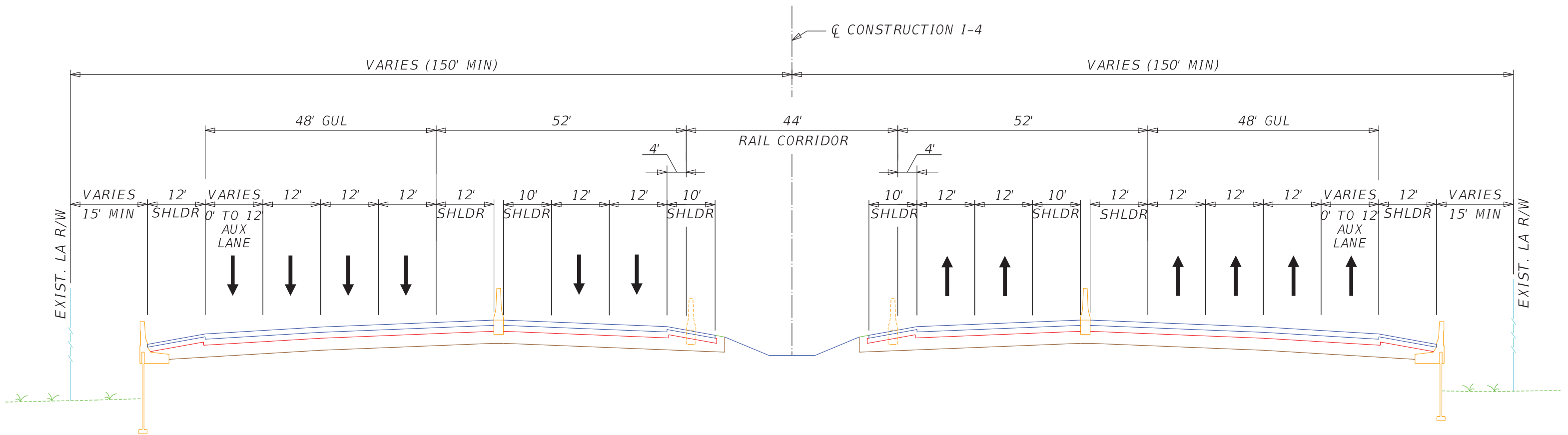
TYPICAL SECTION SR 400 (INTERSTATE 4) DESIGN SPEED = 70 MPH
