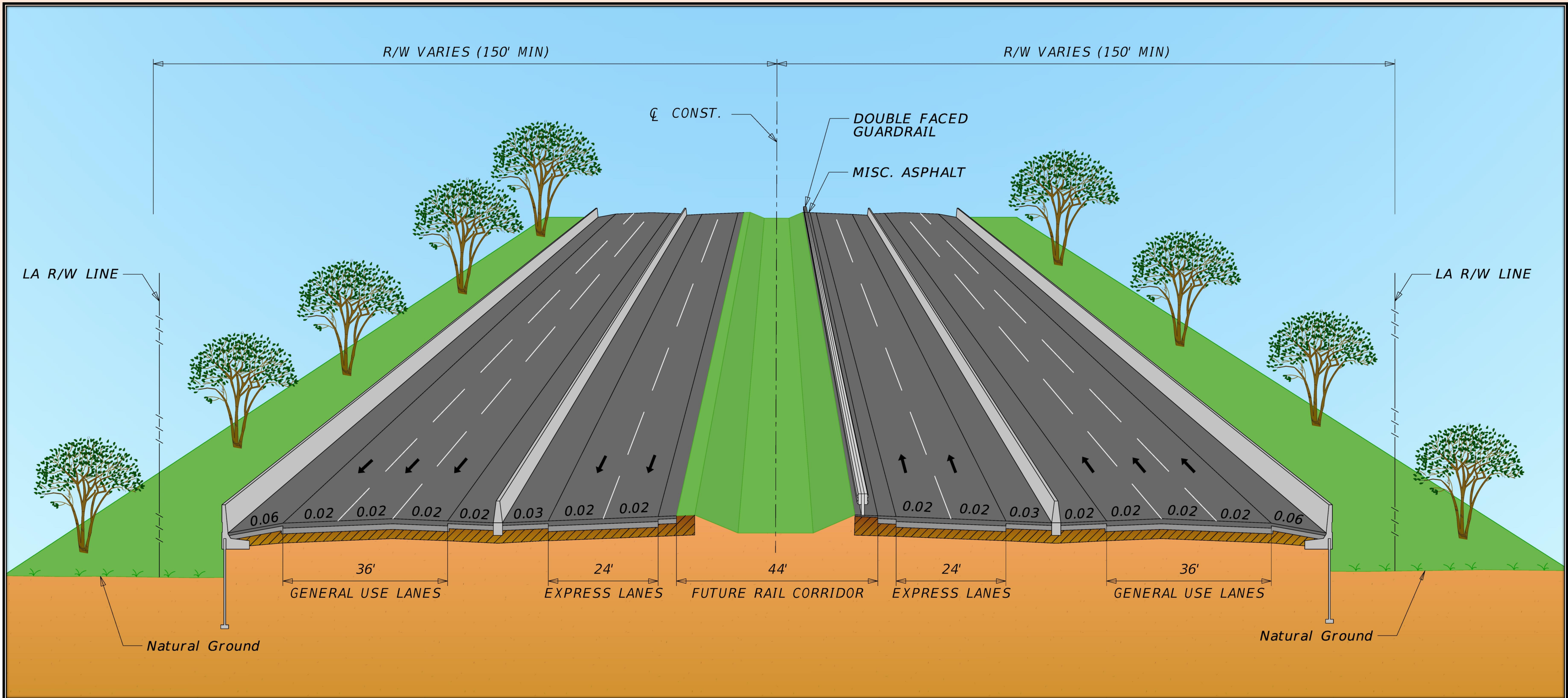
From West of CR 532 to West of SR 528 (Beachline Expressway) (Design Speed = 70 MPH) 6 General Use Lanes + 4 Express Lanes (with Rail Corridor)
